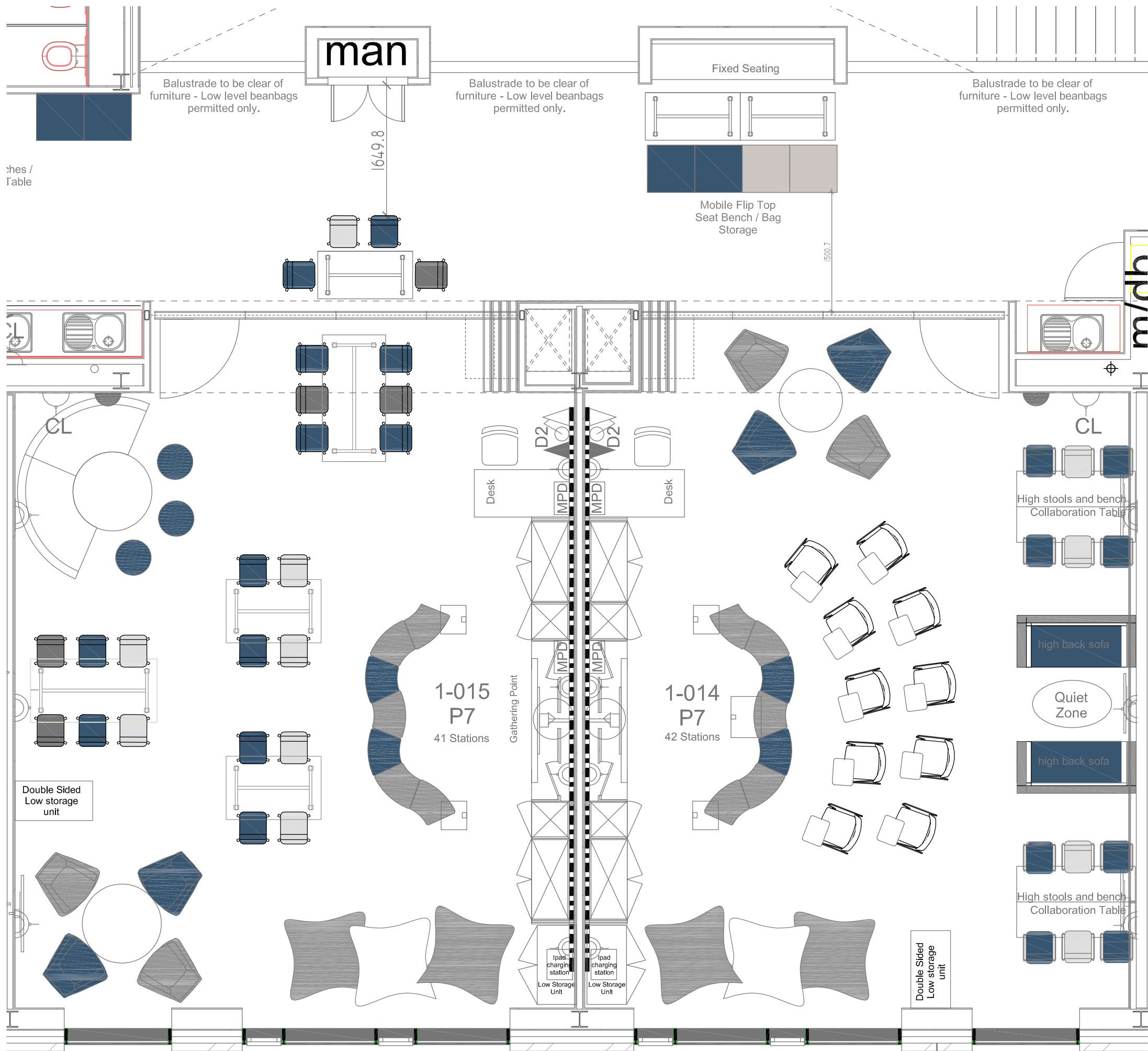
PRIMARY 7 CLASSROOM PLAN: 1:50
